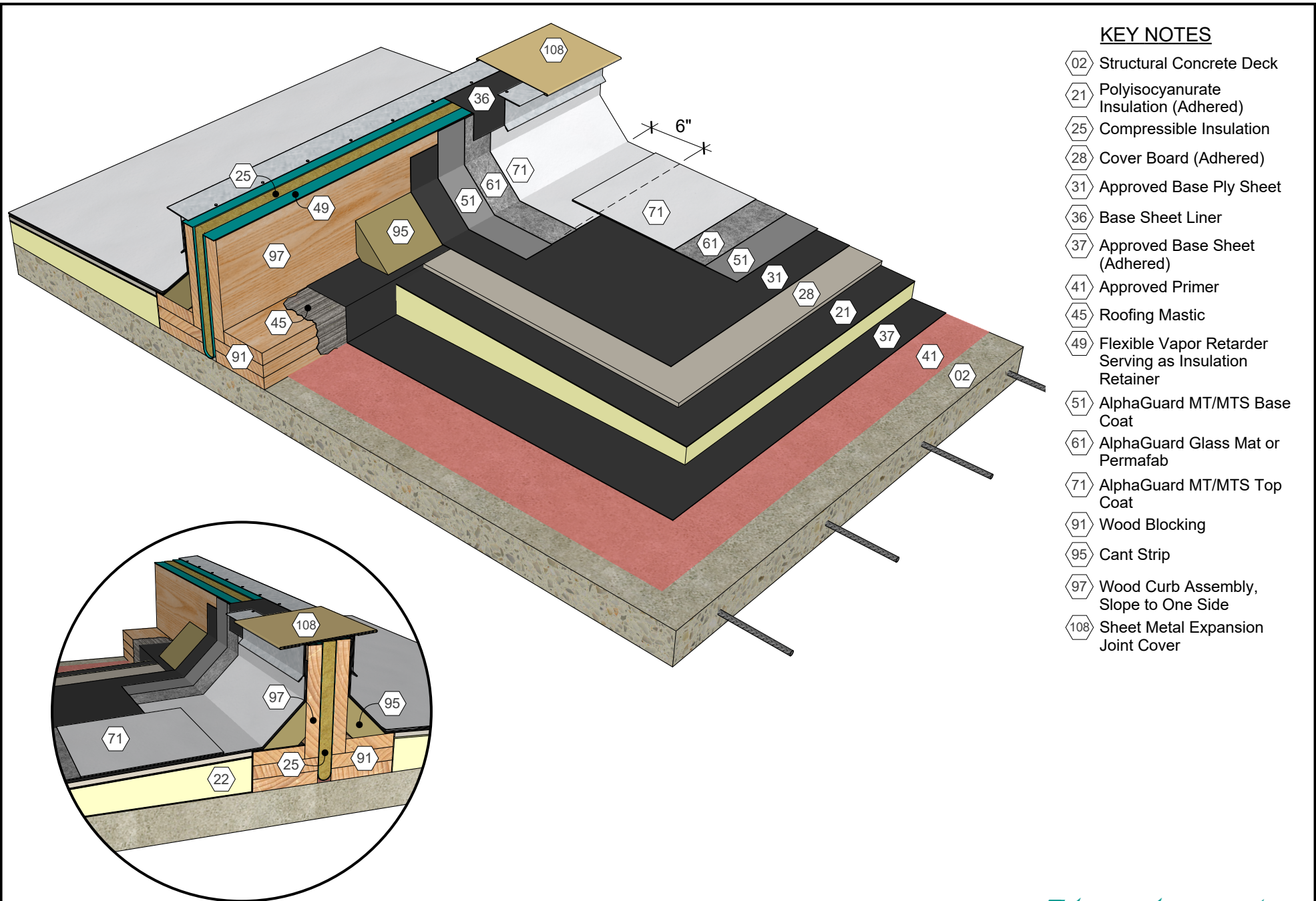
AlphaGuard® MT/MTS Plus Expansion Joint, Temp. Roof, Structural Concrete Deck Detail 32082
