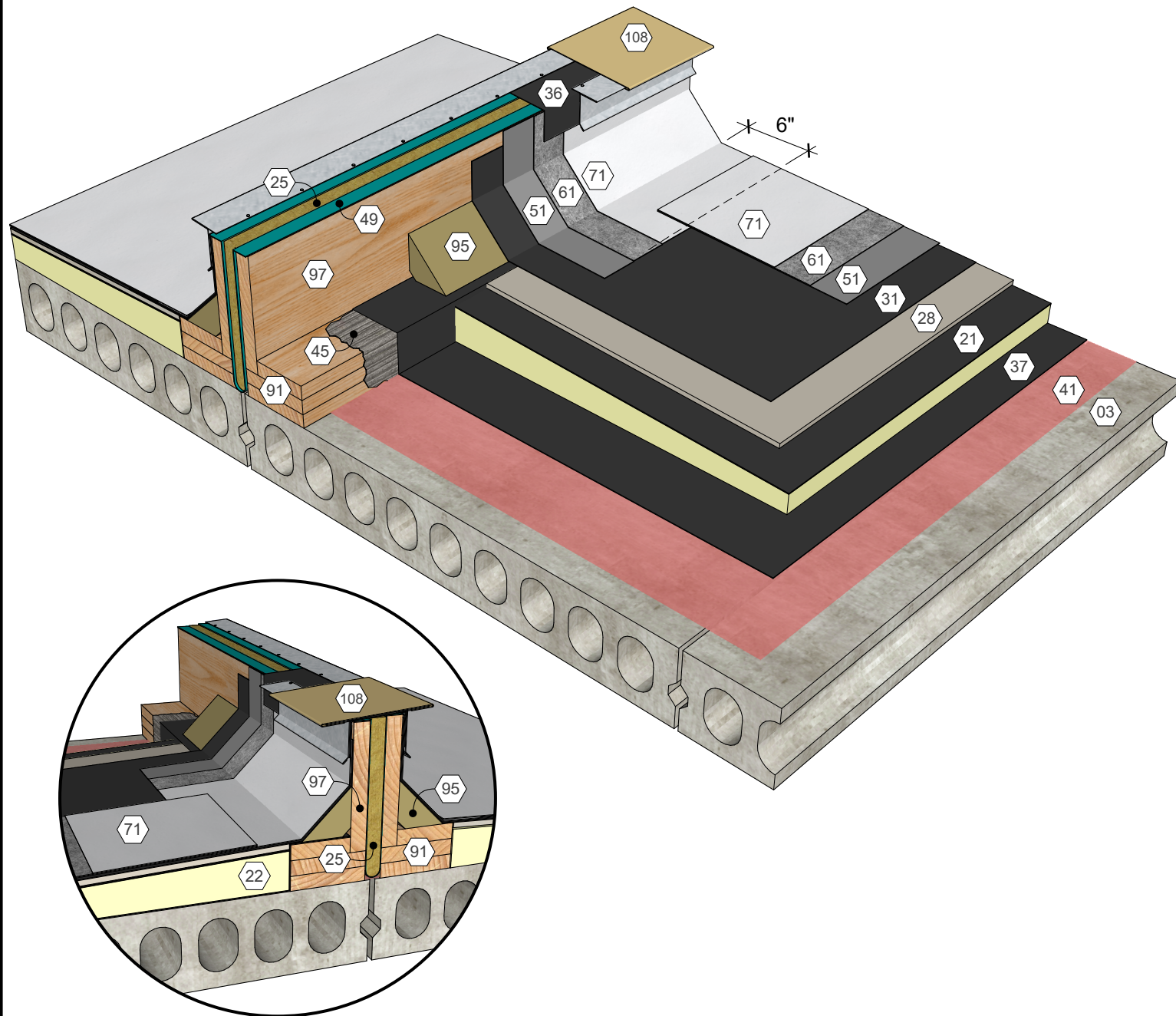
AlphaGuard® MT/MTS Plus Expansion Joint, Temp. Roof, Precast Concrete Deck Detail 32083
